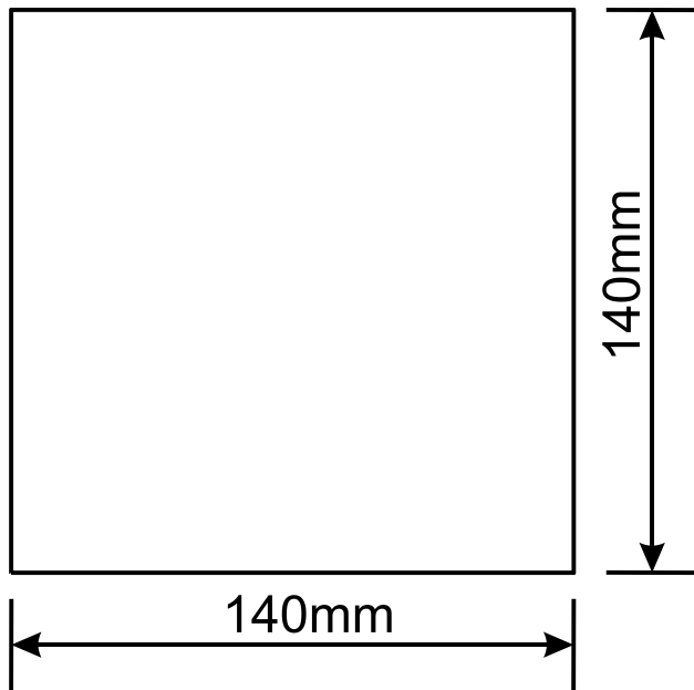
Panel Cutout
